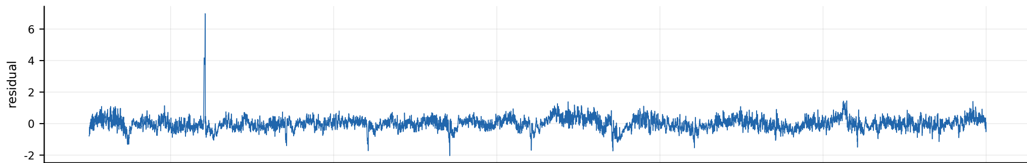
Innovation \eta(t) (whitened)
