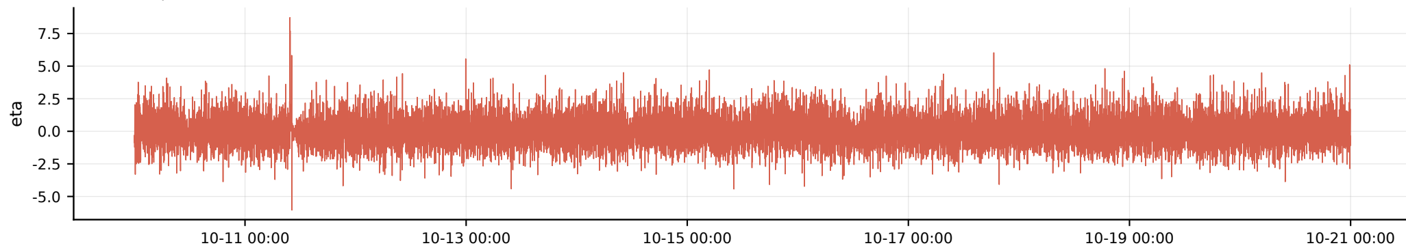
Innovation \eta(t) (whitened)
